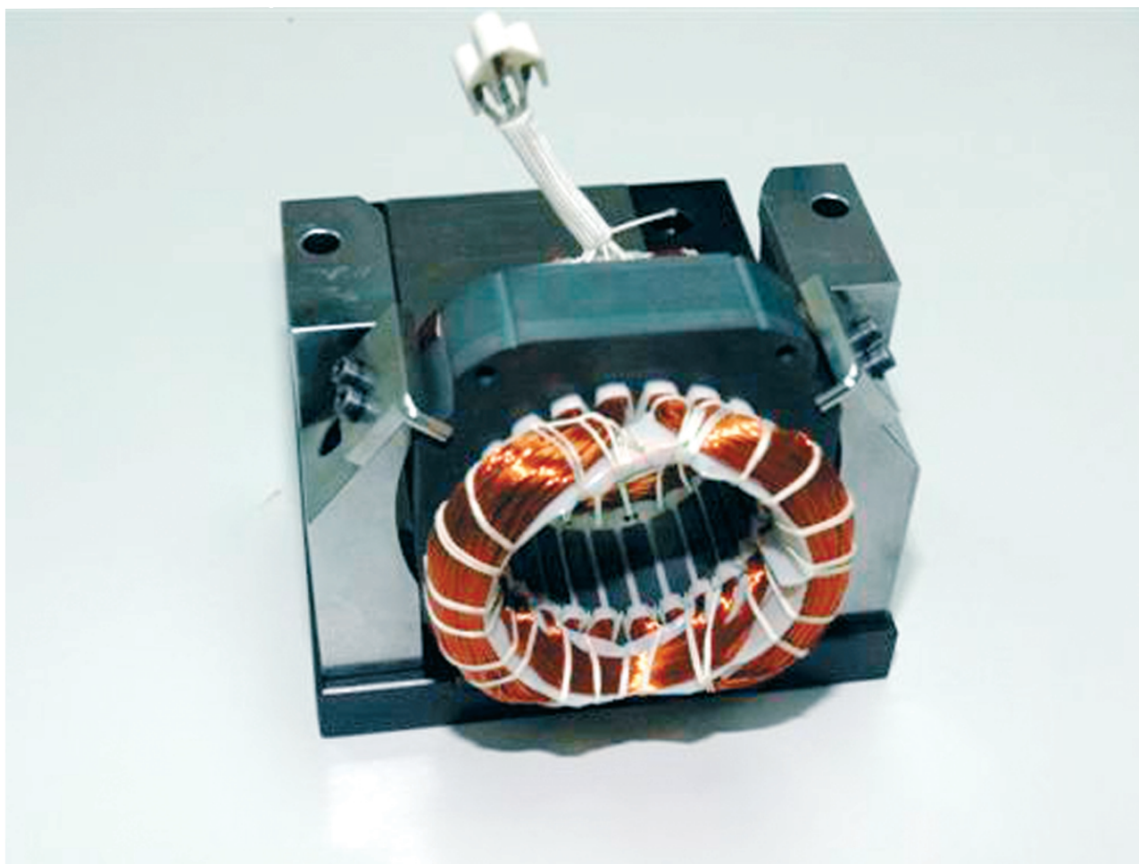
LACING TOOL STATOMAT BN 1
